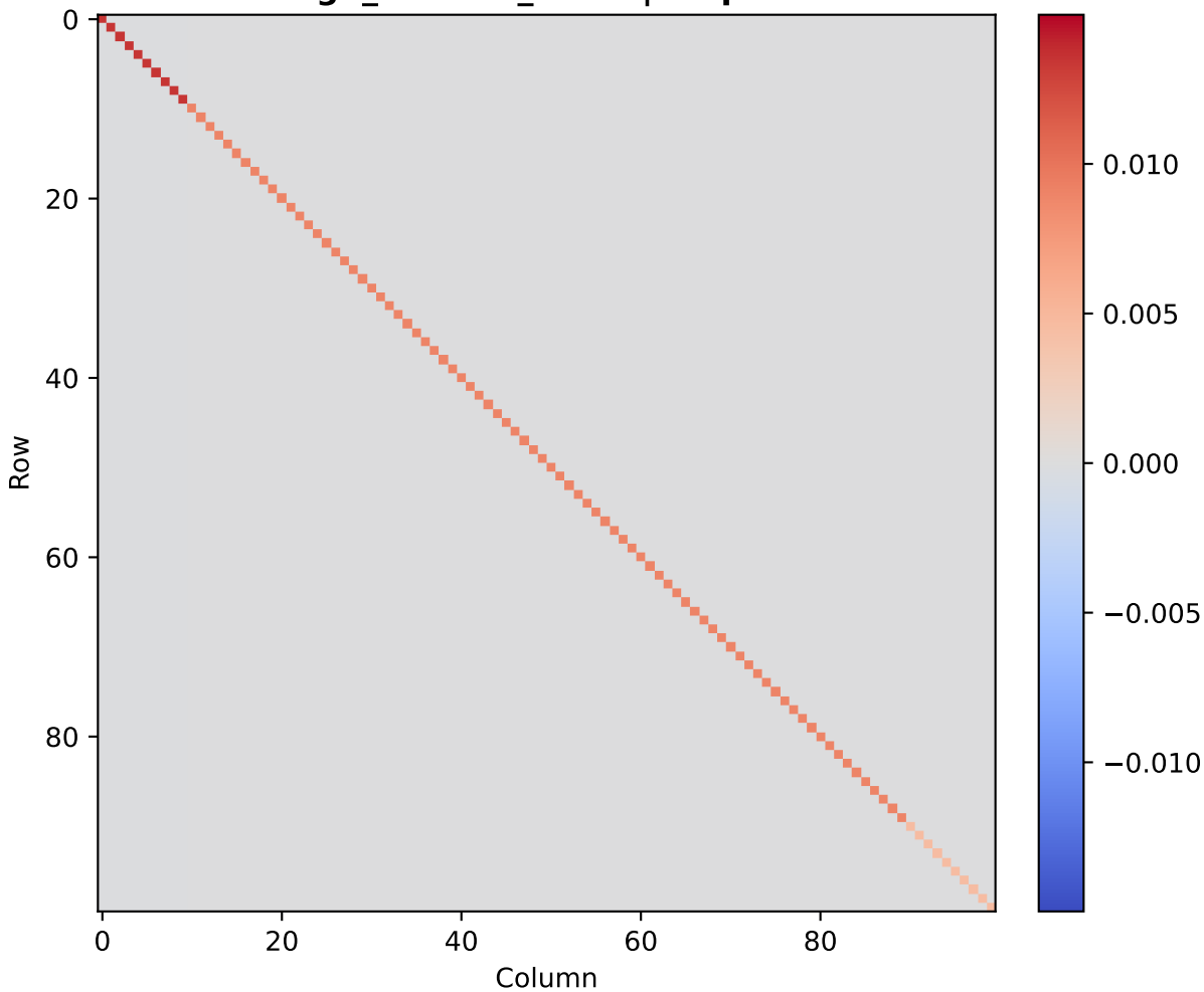
gd_random_small | step 1
